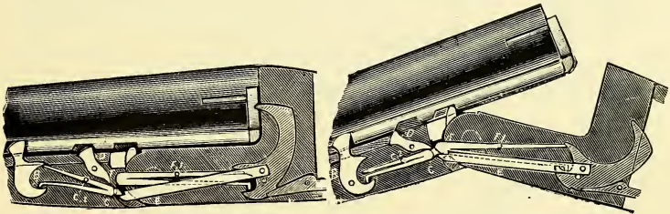
Perkes's Ejector—Gun Fired.
